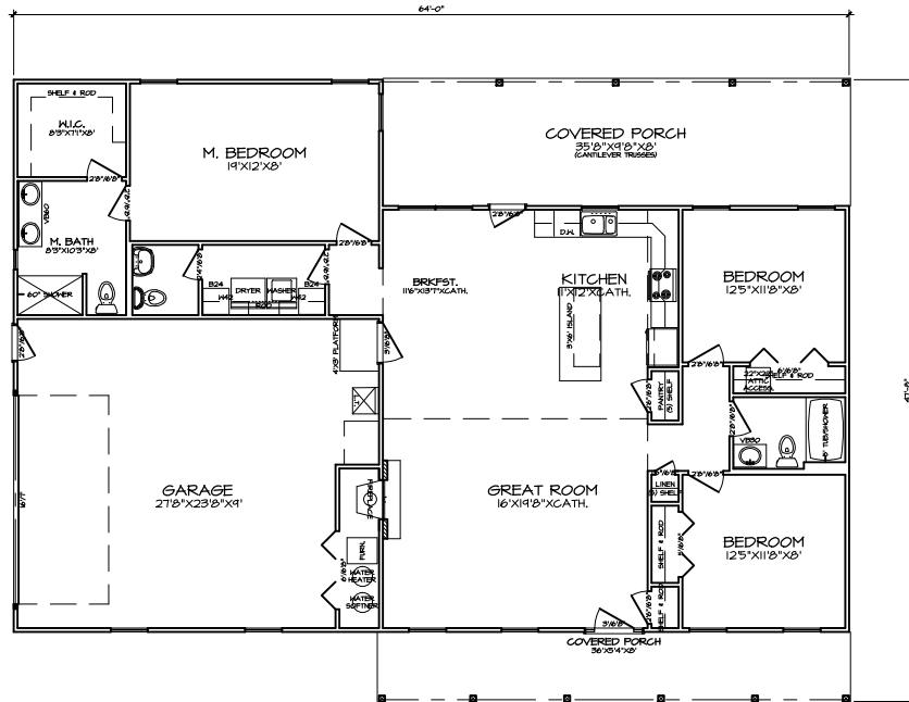
1 FIRST FLOOR PLAN A-4
